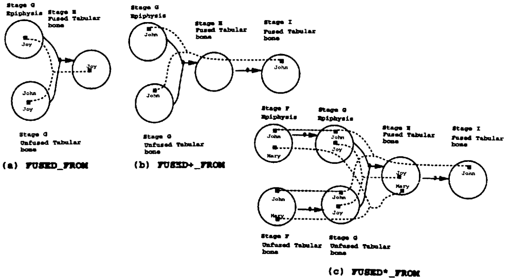
Figure 13. Fusion operators
